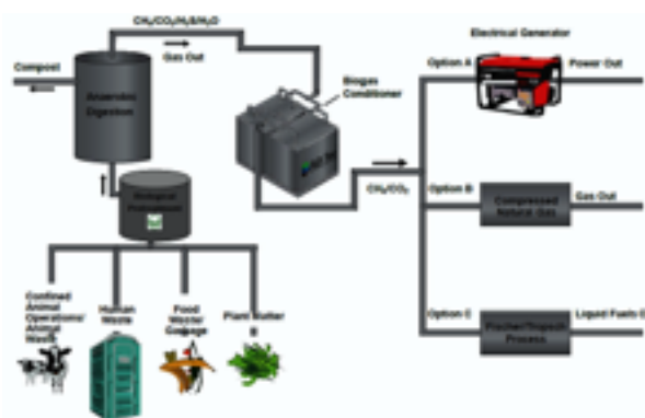
Figure 1: System diagram for biological pretreatment followed by anaerobic digestion for biogas production from waste.
